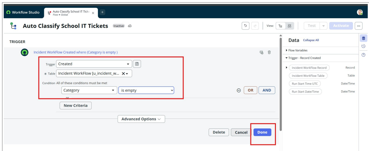
Flow trigger – Record Created on Incident WorkFlow, Category is empty
